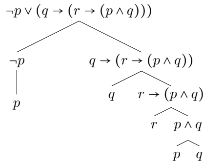
Figure 7.1: An example parse tree.
