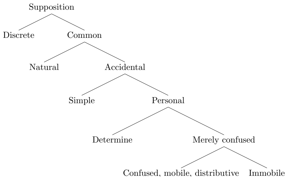
Figure 3.4: Peter’s division of types of suppositio .
