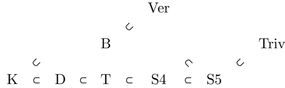
Figure 11.18: Inclusion relations of systems so far
