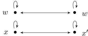
Figure 11.14: An S5 frame where R is not universal
