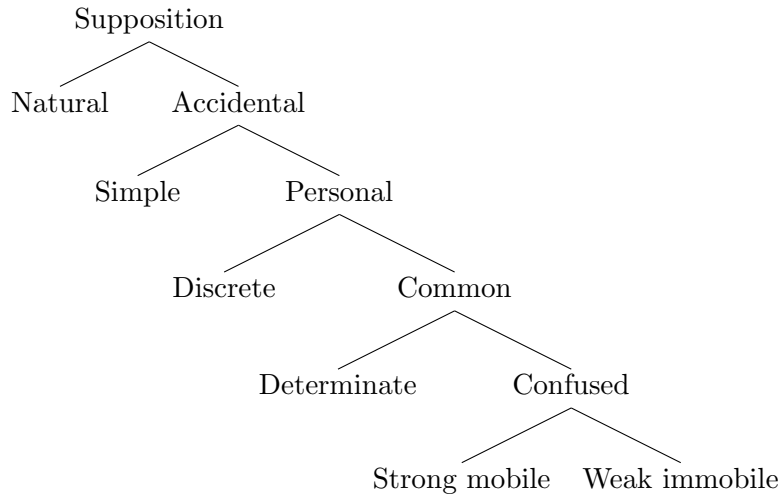
Figure 3.2: Lambert's division of types of suppositio .
