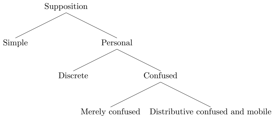
Figure 3.3: Bacon's division of types of suppositio .
