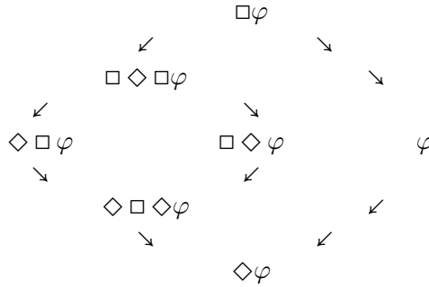
Figure 11.12: Implication relations of positive modalities in S4.
