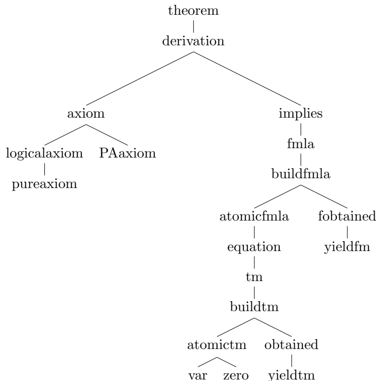
Figure 10.1: A road map to incompleteness.
