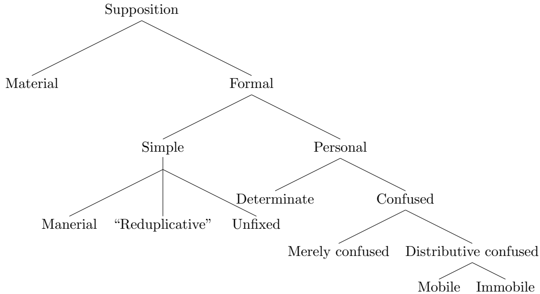
Figure 3.1: Sherwood’s division of types of suppositio .
