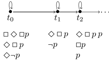
Figure 13.5: Parry's axiom is falsified on a Diodorean matrix
