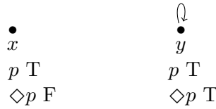
Figure 11.4: The non-truthfunctionality of modal truth
