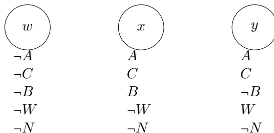
Figure 3.8: A minimal model.
