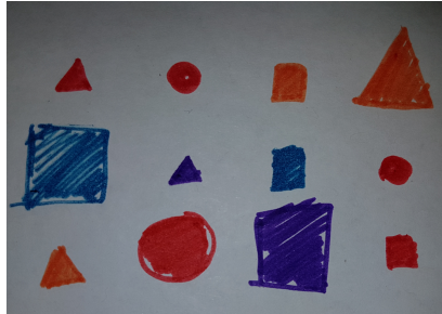
Figure 8.3: Domain for Example 8.2.25
